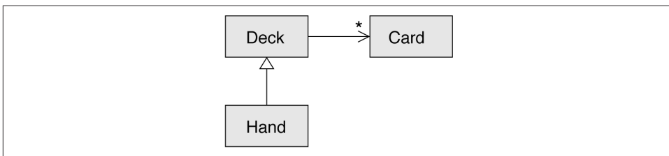
Figure 18-2. Class diagram.
